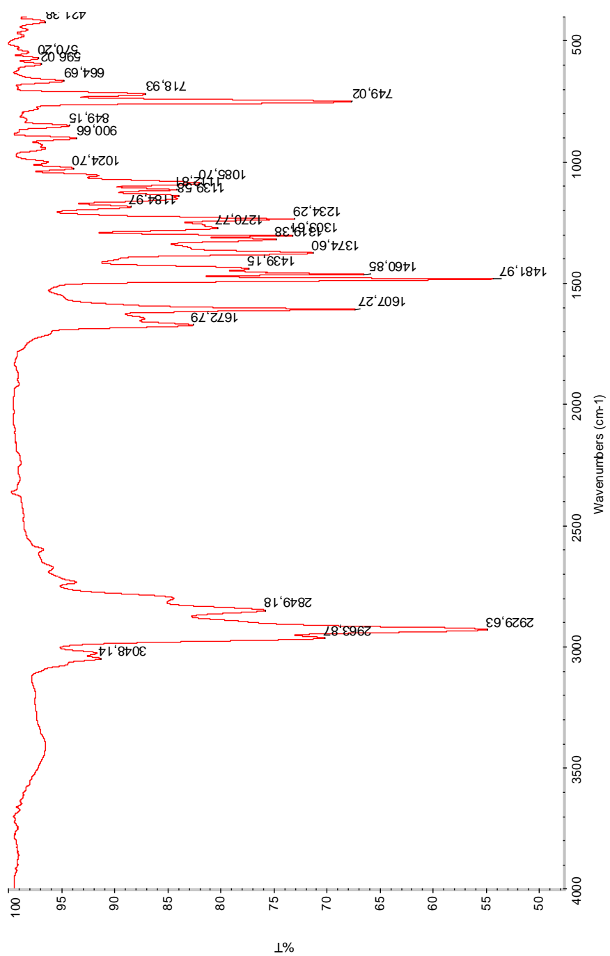
Figure 50: IR spectrum of (AZ-4).
